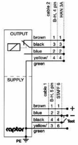
Relay without IR-detection
