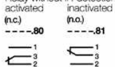
Relay without IR-detection
