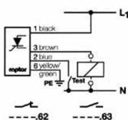
AC test circuit
