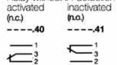
Relay without IR-detection
