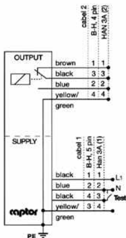
Relay without IR-detection
